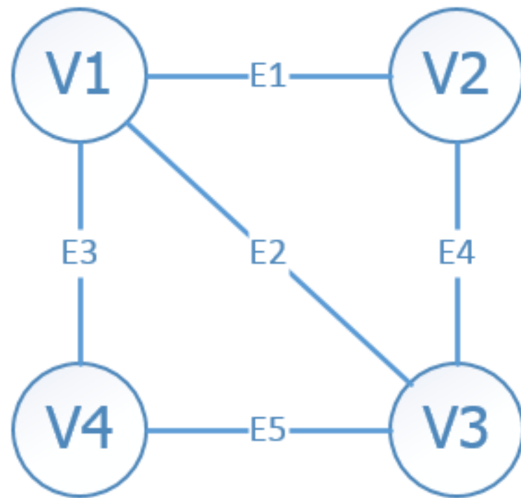
Undirected Graph
